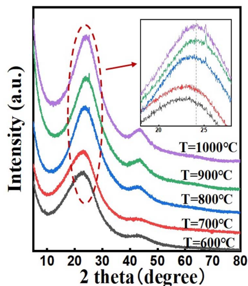
Fig. 1 XRD patterns of the various samples.
