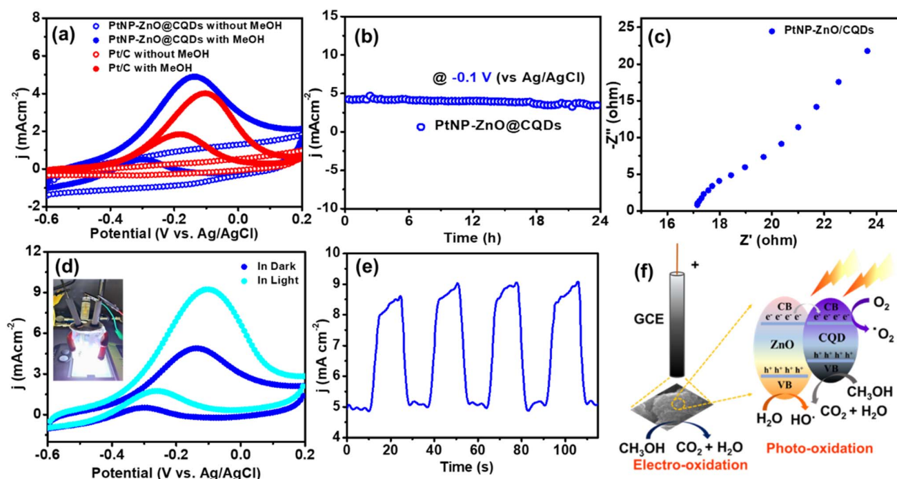
Fig. 3 (a) CV plots of PtNP-ZnO@CQDs and commercial Pt/C modified GCE with and without 1 M methanol in 1 M KOH at a scan rate of 20 mV s^{-1} . (b) Chronoamperometry and (c) Nyquist plot of the PtNP-ZnO@CQD modified GCE with 1 M methanol in 1 M KOH. (d) CV plot of the PtNP-ZnO@CQD modified GCE with 1 M methanol in 1 M KOH at a scan rate of 20 mV s^{-1} in the presence and absence of white LED light. The instrument setup image is given in the inset. (e) Chronoamperometry study of the MOR system under dark and light switching conditions. (f) Band diagram of ZnO and CQDs for the photoinduced electrocatalytic MOR.
