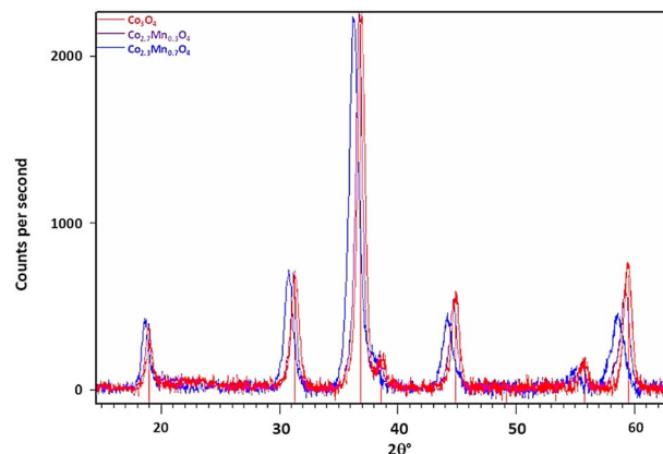
Fig. 1 Background subtracted diffraction patterns of Co_3O_4 and mixed oxide samples Co_{2.7}Mn_{0.3}O_4 (1 wt% Mn) and Co_{2.3}Mn_{0.7}O_4 (3 % wt% Mn) with indexing lines for Co_3O_4 reflections at the bottom. Note the shift of Bragg reflections to lower 2\theta angles with increasing [Mn].
