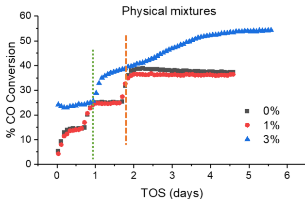
Fig. 10 Activity profile of physical mixture model catalysts throughout testing, with temperature increases from 220–230 °C (green dotted line) for each catalyst, and temperature increase from 230–240 °C (orange dashed line) for 0 and 1% Mn catalysts only. Note Time On Stream (TOS).
