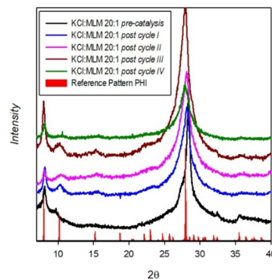
Fig. 1 XRD patterns of the as-obtained PHI (black line), after the first photocatalytic cycle (blue line), after two photocatalytic cycles (pink line), after three photocatalytic cycles (dark red line), after four photocatalytic cycles (green line), and the reference pattern of PHI (red line).
