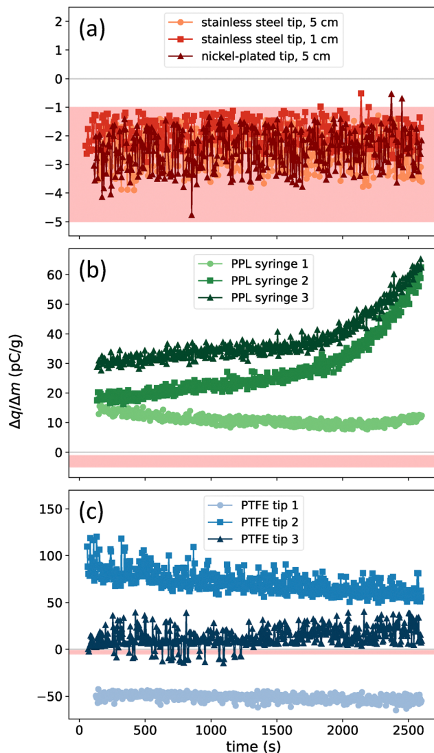
Fig. 7 Time series of \Delta q / \Delta m for different syringe and tip components using 15 mL of DI water at a flow rate of 350 \mu\text{L min}^{-1} . The expected \Delta q / \Delta m range of -5 \text{ pC g}^{-1} to -1 \text{ pC g}^{-1} for metal and glass is highlighted by the translucent red region on each plot. Vertical axis limits vary between plots to better depict the magnitude of \Delta q / \Delta m . (a) Plot of \Delta q / \Delta m versus time for drops dispensed from glass syringe with different metallic syringe tips. Experiments were performed between 30 and 48% RH. The tip length varied, yet all tips had a 2.69 mm ID. Across these experiments, \langle \Delta m \rangle = 0.045 \pm 0.002 \text{ g} . (b) Plot of \Delta q / \Delta m versus time for drops dispensed from stainless steel tips mounted on PPL syringe bodies. All tips had a length of 5 cm and 1.70 mm ID, and experiments were performed at 46% RH. Across these experiments, \langle \Delta m \rangle = 0.0347 \pm 0.0005 \text{ g} . (c) Plot of \Delta q / \Delta m versus time for drops dispensed from PTFE tips mounted on a glass syringe body. All tips were cut to a length of 2 cm before Neutrad cleaning and had a 1.35 mm ID, and experiments were performed at < 30\% RH. Across these experiments, \langle \Delta m \rangle = 0.0267 \pm 0.0005 \text{ g} . Overall, the introduction of plastic components reveals time and history dependent charging behavior.
