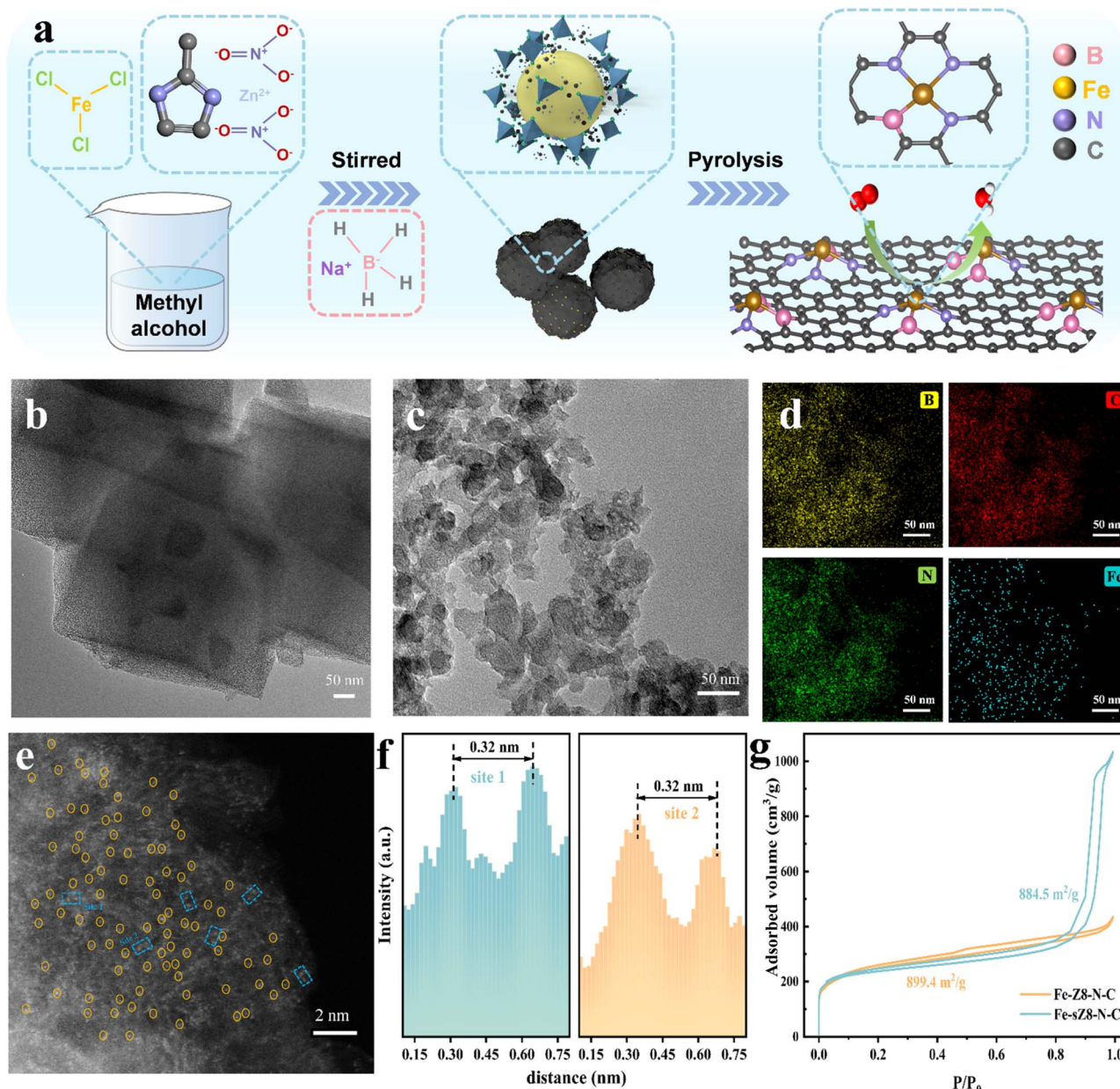
Fig. 1 (a) Schematic illustration of the preparation of the Fe-Z8-N-C catalyst. (b) TEM image of Fe-Z8-N-C and (c) Fe-sZ8-N-C. (d) EDS mapping of Fe-Z8-N-C. (red: C, green: N, yellow: B, and blue: Fe). (e) HAADF-STEM image of Fe-Z8-N-C, the Fe single atoms and paired Fe atoms are marked by yellow circles and blue rectangles, respectively. (f) The corresponding intensity profile of sites 1 and 2 in (e). (g) N_2 adsorption-desorption isotherm of Fe-Z8-N-C and Fe-sZ8-N-C.
