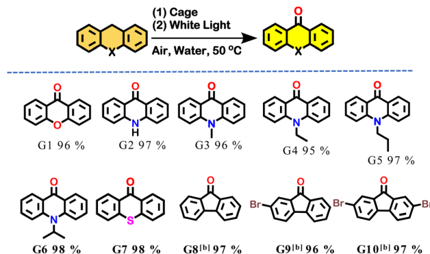
Fig. 6 Scope of the aqueous cage 1 catalyzed \text{C}(\text{sp}^3)\text{--H} oxidation of alkylarenes. The yield is calculated by ^1\text{H} NMR using 1,3,5-trimethoxybenzene as an internal standard [b: a 390 nm 100 W LED was used]. The % conversion was calculated by ^1\text{H} NMR using the internal standard 1,3,5-trimethoxybenzene.
