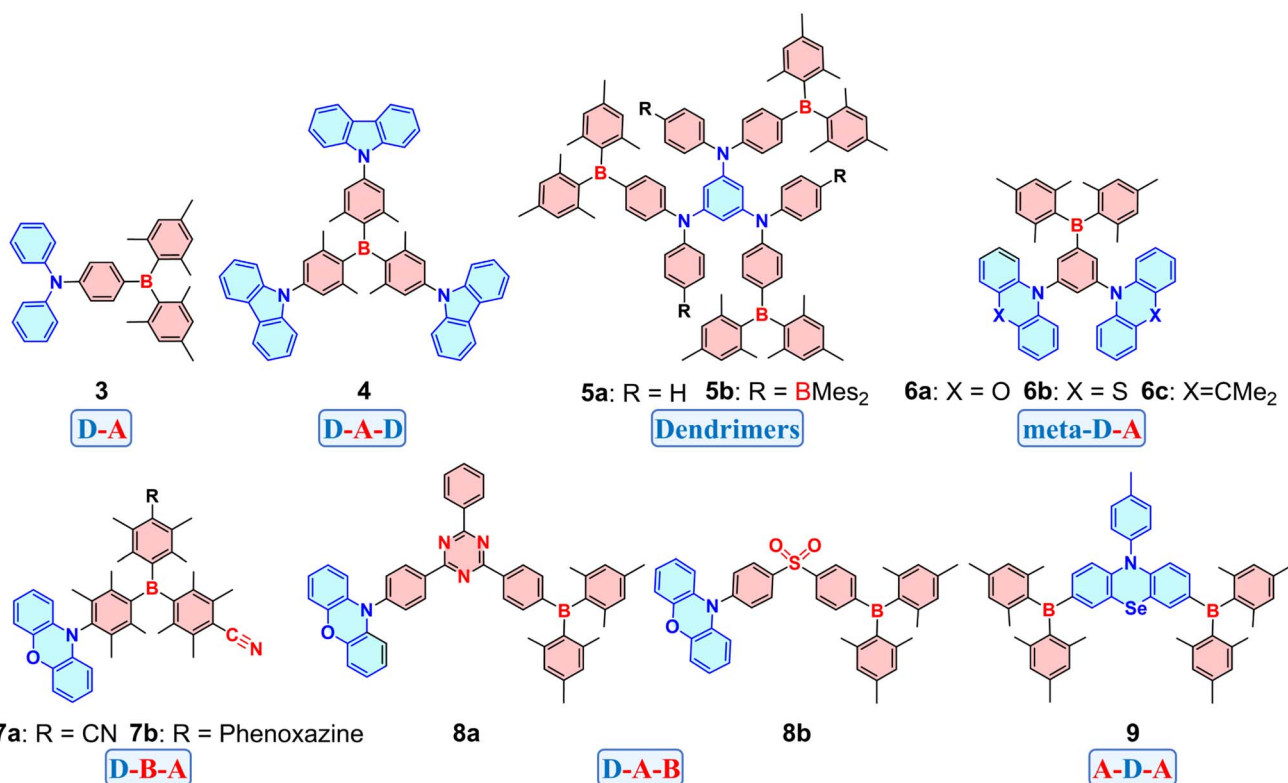
Fig. 5 Representative D-A OBCTs with unbridged triarylboron acceptors.
