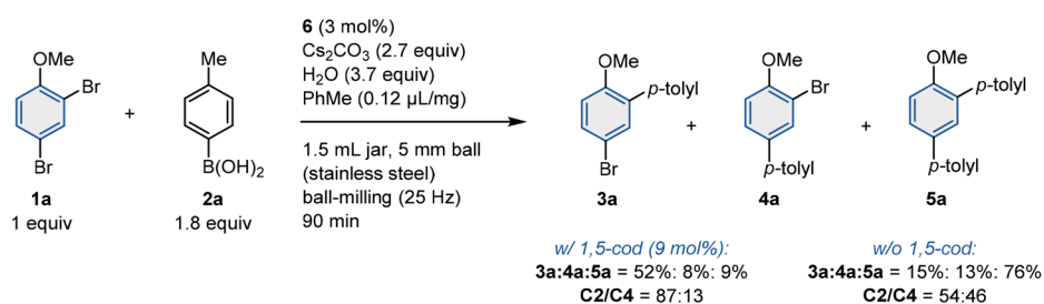
Scheme 4 Synthesis and reactivity of the oxidative-addition complex 6.
