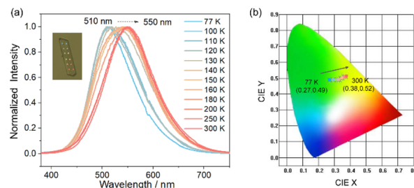
Fig. 4 (a) PL spectra of compound 1DySeCN with increasing temperature ( \lambda_{\text{ex}} = 375 nm), inset: single crystal samples used for measurement and test positions at different temperatures; (b) the CIE graph of 1DySeCN in the range 77–300 K.
