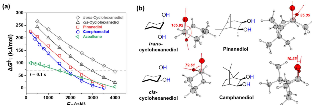
Fig. 3 (a) Computed \Delta G^\ddagger_\tau – F\tau graph at the UB3LYP-D3/6-311G(d,p)//UB3LYP-D3/6-311G(d,p) level of theory for the homolytic cleavage of the C–C bond in a series of vicinal diols. The x-axis represents the level of simulated tensile force, while the y-axis indicates the force-coupled free energy barrier for C–C bond cleavage. The \Delta G^\ddagger_\tau – F\tau curve of a conventional mechanophore, azoalkane, is also included as a reference. (b) Optimised structures of the force-coupled transition states under F\tau = 2000 pN, highlighting the presence of a “node” in camphanediol, characterised by an O–C–C–O dihedral angle of 10.55°.
