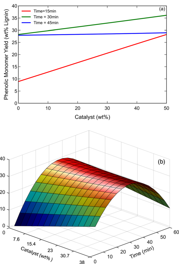
Fig. 9 The interaction effect of catalyst and time on phenolic monomer yield (a) two-dimensional (b) three-dimensional (response surface). Regression models were produced while keeping other explanatory variables constant at their center point (temperature: 170 °C, O 2 pressure: 120 psi, NaOH: 1.25 M).
