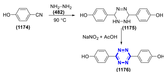
Scheme 326 Synthesis of tetrazines under catalyst-free conditions.
