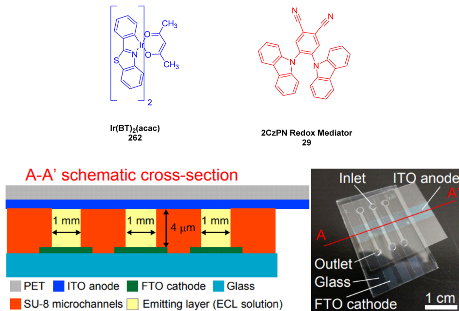
Fig. 104 Molecular representation of 2CzPN (29) and \text{Ir(BT)}_2(\text{acac}) (262) along with the microfluidic ECL cell with a schematic cross-section. Reproduced from ref. 309, https://doi.org/10.5796/electrochemistry.23-00147 , under the terms of the CC BY 4.0 license, https://creativecommons.org/licenses/by/4.0/ .
