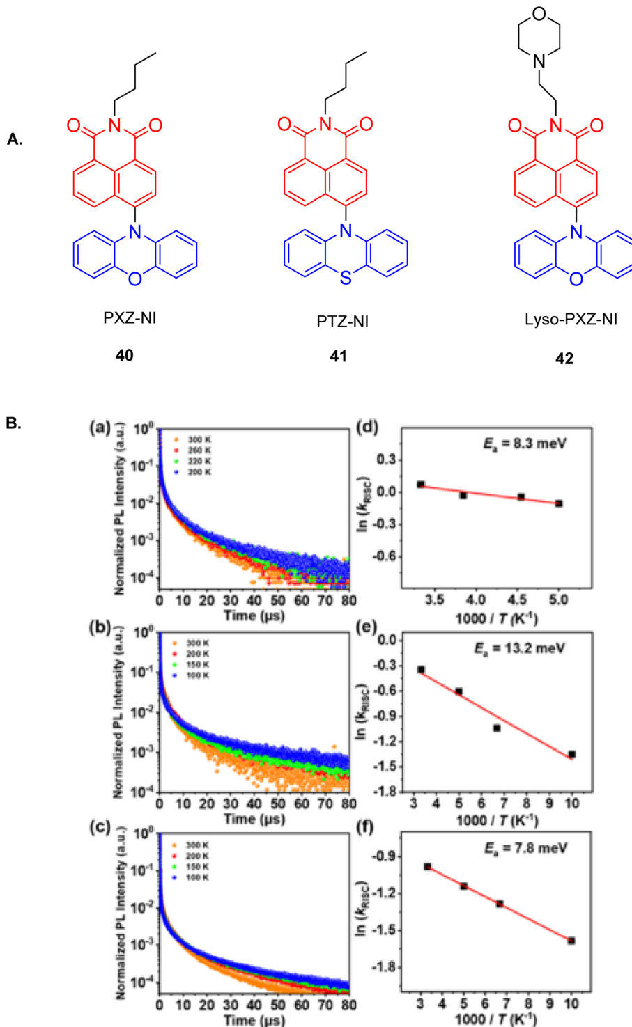
Fig. 18 (A) Structures of TADF organic materials PXZ-NI ( 40 ), PTZ-NI ( 41 ), and Lyso-PXZ-NI ( 42 ). (B) Temperature-dependent TRPL signals for (a) PXZ-NI ( 40 ), (b) PTZ-NI ( 41 ), and (c) Lyso-PXZ-NI ( 42 ), and corresponding Arrhenius plots for the TRPL signals for (d) PXZ-NI ( 40 ), (e) PTZ-NI ( 41 ), and (f) Lyso-PXZ-NI ( 42 ). Reproduced from ref. 165 with permission from American Chemical Society, Copyright © 2020.
