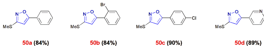
Scheme 15 Synthesis of 3-methylthio-5-aryl-isoxazoles 50 .
