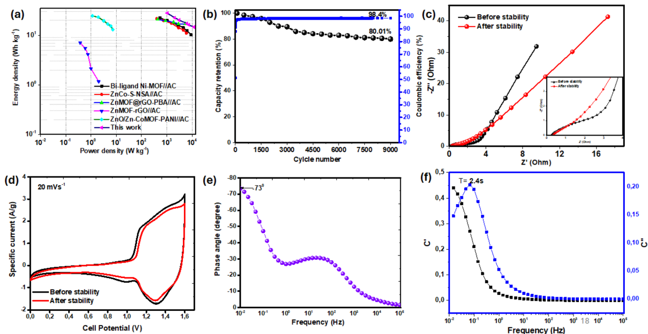
Fig. 14 (a) Ragone plot of the device, (b) cycling stability test after 10 000 cycles at 10 A g -1 , (c) Nyquist plot with an inset showing high frequency zone magnification before and after cycle stability, (d) CV plots before and after stability, (e) Bode plot and (f) imaginary and real capacitance vs. frequency of the hybrid device.
