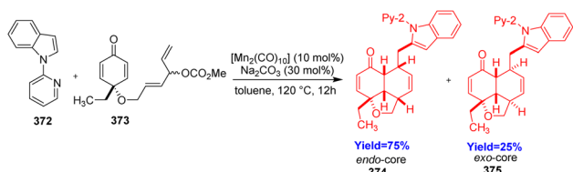
Scheme 47 Synthesis of 6/6/5-fused tricyclic terpene scaffold. 101
