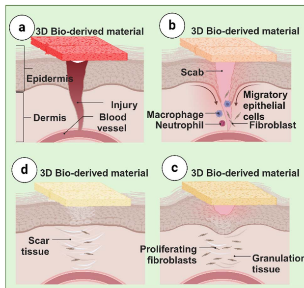
Fig. 1 Different phases in wound healing – [a] bleeding and hemostasis, [b] inflammation, [c] proliferation, and [d] remodeling. Created in BioRender. Dhillip Kumar S. (2025) https://BioRender.com/q39h755 .
