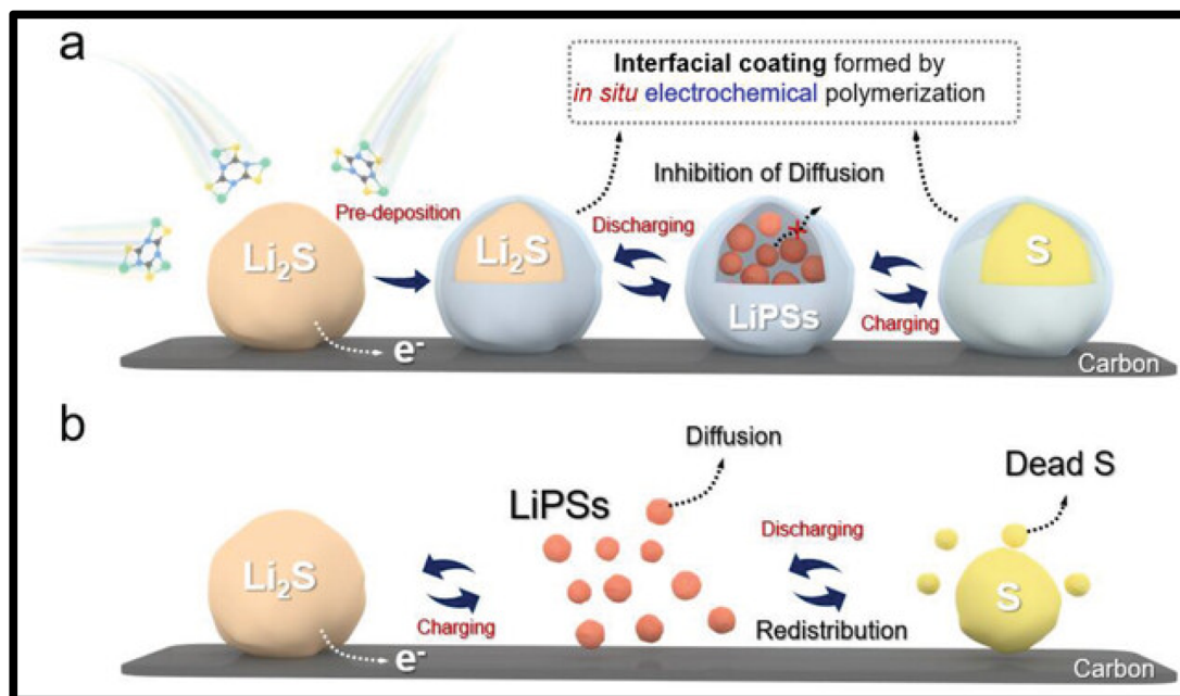
Fig. 8 Schematic of in situ coating Li 2 S with polymerizable electrolyte additive. (a) The soluble TTCA-Li electrochemically polymerizes on the Li 2 S surface to form a POS coating during the initial charging, which inhibits the out-diffusion of LiPSs during subsequent cycling. (b) Li 2 S cathodes without TTCA-Li additive generate soluble LiPSs and undergo uncontrollable sulfur redistribution during cycling. 142
