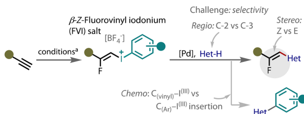
Fig. 1 The importance of monofluoroalkenes, the fluorovinylation of indoles at C-2 and our strategy for achieving β-fluorovinylation using fluorovinyl iodonium (FVI) salts. a See ESI† and ref. 15.
