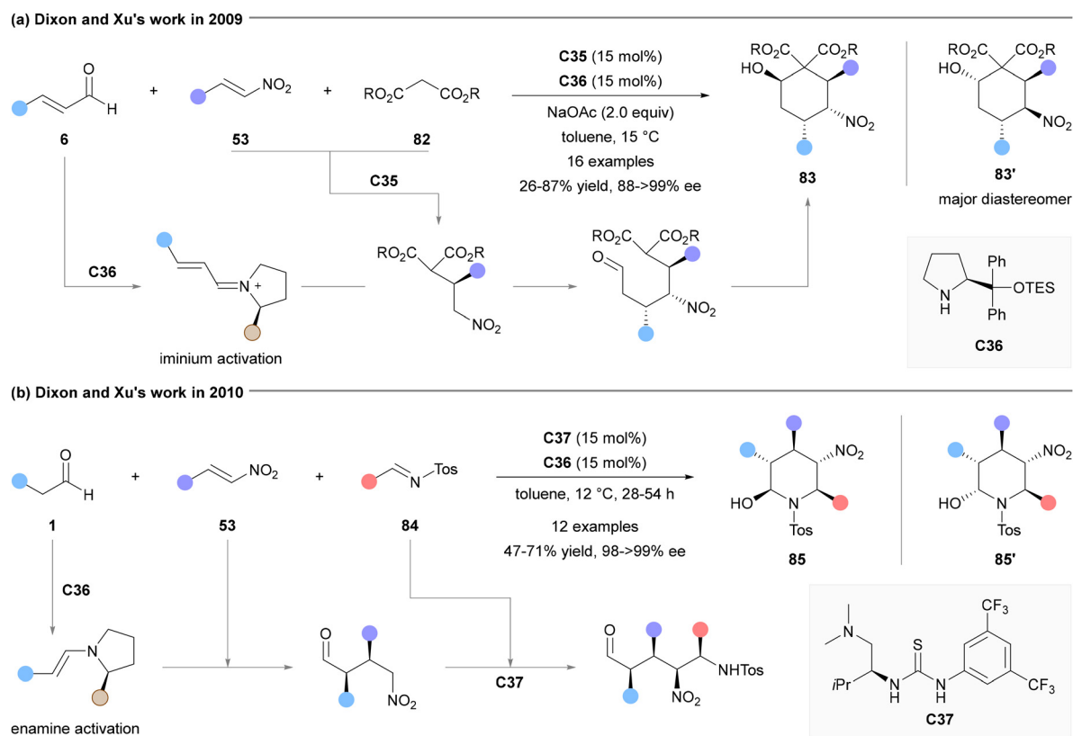
Fig. 19 AMCRs towards substituted six-membered cycles catalyzed by chiral thiourea.
