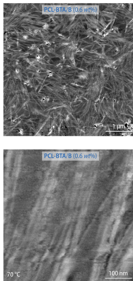
Fig. 6 Intermittent-contact AFM phase images of PCL-BTA/B (0.6 wt%) recorded at 70\text{ }^{\circ}\text{C} at different magnifications. See ESI Fig. S13 ^{\dagger}
