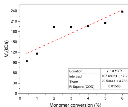
Fig. 1 Linear regression of M_n vs. monomer conversion determined by ^1\text{H} NMR spectroscopy at room temperature using 0.1 mol% (\text{LaCl}_3/[\text{Cu}(\text{CH}_3\text{CN})_4]\text{PF}_6) as catalyst.
