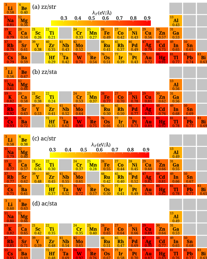
Fig. 4 Interface energies. Heat maps of interface energies calculated using ML for a) zigzag/straight, b) zigzag/staggered, c) armchair/straight, and d) armchair/staggered interfaces, corresponding to minimum lattice mismatch. The interface energies are shown under each element.
