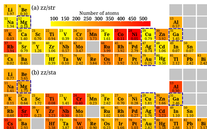
Fig. 2 Heat maps of number of atoms for modeled zigzag graphene-metallene interfaces based on selection criteria. a) zigzag/straight and b) zigzag/staggered interfaces. The lattice mismatch (strain in graphene) is shown under each element name. The metals selected for DFT calculations are highlighted by dashed boxes.
