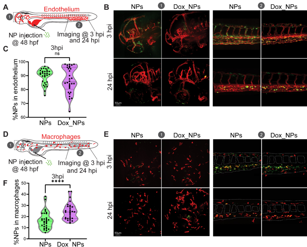
Fig. 3 Biodistribution of HSA NPs and their interaction with endothelial cells and macrophages. (A) Description of the experimental setup: 48 hour post-fertilization (hpf), Tg(Kdr1.hsa-HRAS:mCherry) zebrafish embryos (endothelial cells in red) were injected intravascularly via the duct of Cuvier with both NPs and DOX-containing NPs (Dox_NPs) surface-modified with HSA-FITC. Embryos were imaged in the head (1) and caudal plexus area (2) 3 or 24 hour post-injection (hpi). Representative images (B) of the NPs in the head (1) and caudal plexus (2) areas, and quantification of the NPs colocalized with the endothelium (C). At 3 hpi, there is no difference between the NP and Dox_NP injected groups (Mann–Whitney test, 3 independent experiments, and 30 embryos in total). (D) Description of the experimental setup: 48 hour post-fertilization (hpf), Tg(mpeg-ntr:mCherry) zebrafish embryos (macrophages in red) were injected intravascularly via the duct of Cuvier with both NPs and DOX-containing NPs (Dox_NPs) surface-modified with HSA-FITC. Embryos were imaged in the head (1) and caudal plexus area (2) at 3 or 24 hpi. Representative images (E) of the NPs in the head (1) and caudal plexus (2) areas, and quantification of the NPs colocalized with macrophages (F). At 3 hpi, Dox_NPs exhibited significantly higher colocalization with macrophages, as compared to the NPs without the drug (Mann–Whitney test, p < 0.0001 , 3 independent experiments, and 30 embryos in total). Scale bar = 50 \mu\text{m} .
