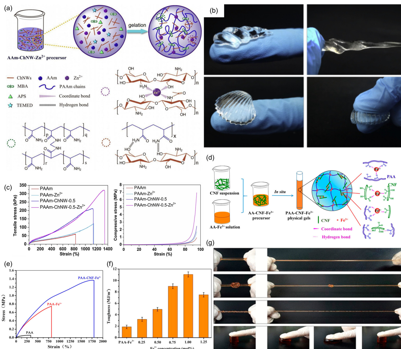
Fig. 25 Mechanical properties of hydrogels enhanced by metal coordination sacrificial bonds. (a) Scheme showing polyacrylamide gels with chitin nanowhiskers and Zn^{2+} ions (PAAm-ChNW- Zn^{2+} ). (b) Different shapes of PAAm-ChNW- Zn^{2+} achieved by twisting and bending. (c) Tensile and compressive stress versus strain curves of PAAm-ChNW- Zn^{2+} gels show that addition of Zn^{2+} increases both tensile strength and toughness. Reprinted from ref. 125 with permission from Elsevier, copyright 2020. (d) Scheme showing the formation of a PAA matrix with cellulose nanofibrils and Fe^{3+} ions (PAA-CNF- Fe^{3+} ). (e) Uniaxial tensile tests reveal enhancement of mechanical properties upon addition of CNF and Fe^{3+} ions. (f) Tensile toughness varies with [Fe^{3+}] in PAA-CNF- Fe^{3+} . (g) PAA-CNF- Fe^{3+} gels can be (from top) stretched, knotted, twisted and compressed. Adapted with permission from ref. 126. Copyright 2017 American Chemical Society.
