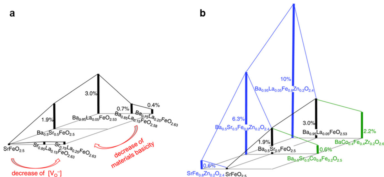
Fig. 8 Proton concentration in perovskite oxides systems of (Ba, Sr, La)(Fe, Co, Zn)O 3-δ system at 250 °C and 16 mbar H 2 O. (a) Effect of A-site cations (Ba, Sr and La) and (b) effect of B-site cations (Fe, Co and Zn). This figure has been adapted from ref. with permission from John Wiley & Sons, copyright 2025.
