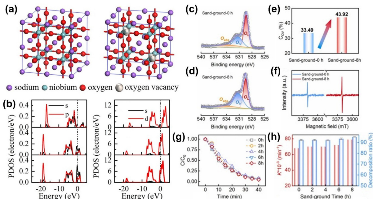
Fig. 6 (a and b) Crystal structures of primitive (left) and 5.6% oxygen vacancy containing \text{NaNbO}_3 (right). (b) PDOS of Na (left) and Nb atoms (right) in the \text{NaNbO}_3 with different oxygen vacancy concentrations of 0%, 2.8%, and 5.8% from top to bottom in each column, respectively. Reprinted with permission from ref. 100. Copyright 2023, Elsevier. (c–e) Comparison of (c and d) XPS spectra of O 1s, (e) concentration of oxygen vacancies, and (f) EPR spectra between KNN samples sand-grounded for 0 h and 8 h. (g) Piezocatalytic RhB degradation of KNN samples prepared using sand-ground at different durations and (h) corresponding reaction rate constant and decomposition rate. Reprinted with permission from ref. 102. Copyright 2023, Elsevier.
