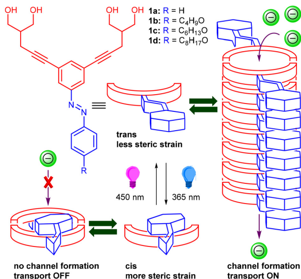
Fig. 1 Schematic representation of the structures of the designed molecules and photoresponsive ion transport through azobenzene-based ion channel structures.
