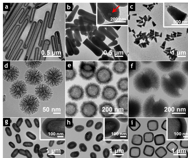
Fig. 4 TEM images of silica particles exhibiting different morphologies: (a) tubular, (b) needle-shaped, and (c) bell-shaped, all obtained by varying the concentrations of ammonia, sodium citrate, polyvinylpyrrolidone, chloroauric acid, and/or NaCl during synthesis. Reprinted with permission. 80 Copyright © 2014, IOP Publishing Ltd. (d) DMSNs exhibiting central-radial pore structure. Reprinted with permission. 81 Copyright © 2013 American Chemical Society. (e) Hollow MSNs with spikes on the surface (silica nanopollens). Reprinted with permission. 82 Copyright © 2016 American Chemical Society. (f) Asymmetric head-tail DMSNs. The dendritic tail grows on spherical particles (head) using an oil/water emulsion system. The length and tail coverage on head particles are adjustable. Reprinted with permission. 83 Copyright © 2017 American Chemical Society. Nonspherical hollow MSNs with controlled morphologies: (g) capsules, (h) rice, and (i) cubes. The mesoporous structure grows by inheriting the original shape of the Fe 2 O 3 templates, which are subsequently removed to obtain hollow particles. Reprinted with permission. 84 © 2017 Wiley-VCH Verlag GmbH & Co. KGaA, Weinheim.
