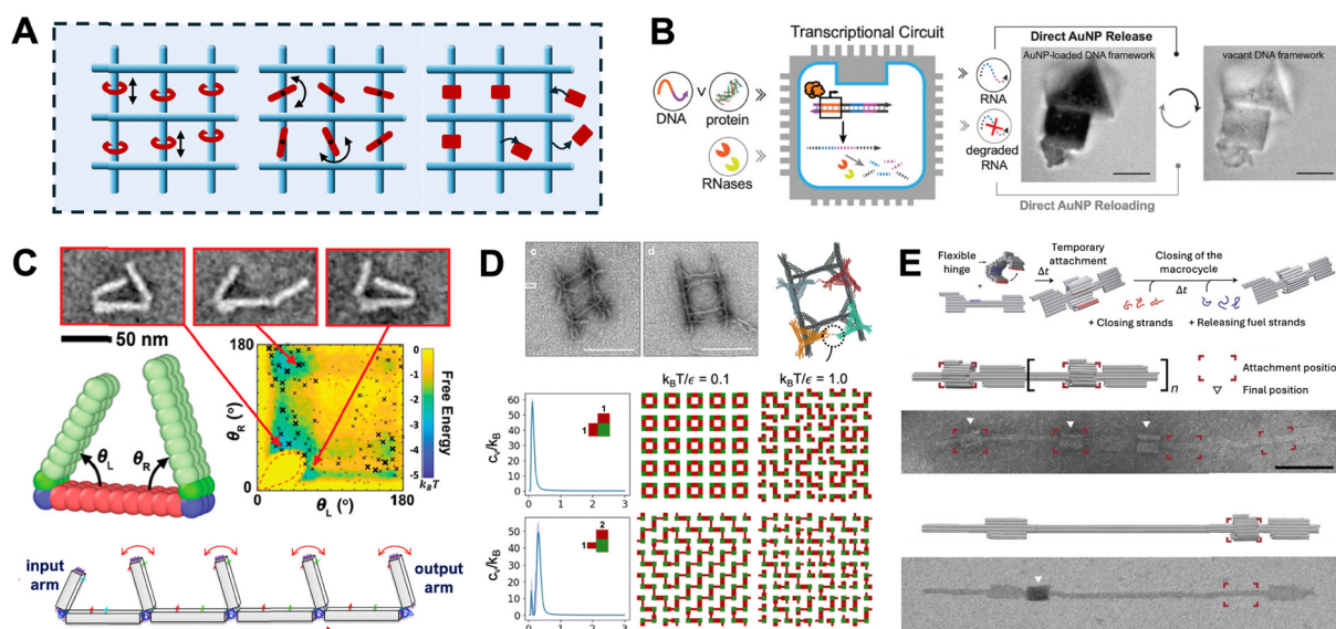
Fig. 5 Static superstructures housing dynamic DNA origami subunits. (A) Schematic of such lattices with translatable, rotatable, and dissociable components. (B) Crystal that loads and unloads gold nanoparticles in response to the output of a transcriptional circuit (reproduced with permission from ref. 68; Copyright 2024, American Chemical Society). (C) TEM images and angle distributions from coarse-grained simulations of minimal unit of a sterically communicating DNA origami array (reproduced with permission from ref. 66; Copyright 2023, American Chemical Society). (D) TEM images of 2 \times 2 rotor lattice and order–disorder transitions of 10 \times 10 lattices as predicted by Monte Carlo simulations (reproduced with permission from ref. 67; Copyright 2023, Royal Society of Chemistry). (E) Method for assembling mechanically interlocked rotaxane-like structures, as well as TEM images showing movement of the dynamic component (reproduced with permission from ref. 16; Copyright 2016, Springer Nature).
