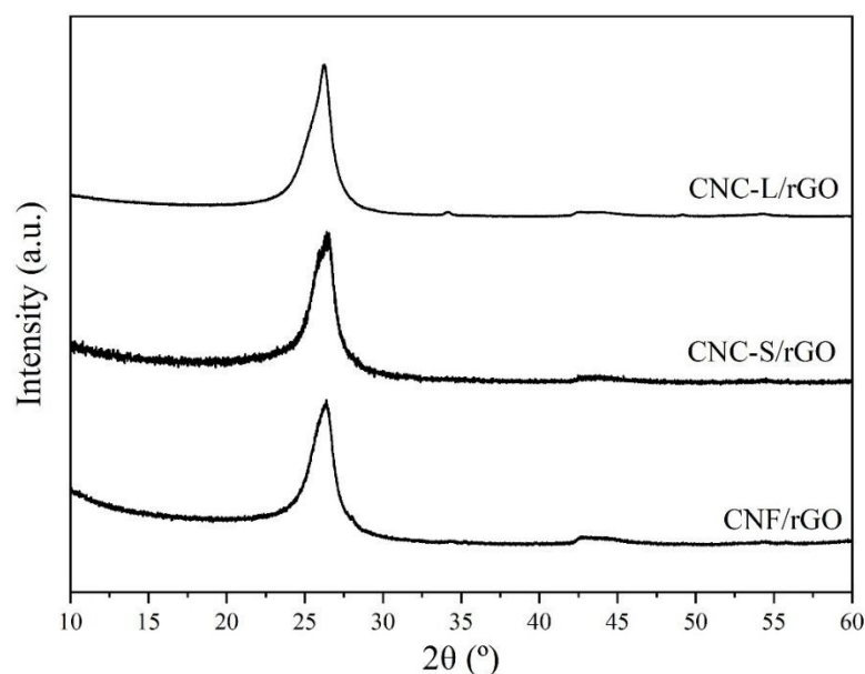
Fig. 2. Wide-angle XRD patterns of CNF/rGO, CNC-L/rGO, and CNC-S/rGO, respectively.
