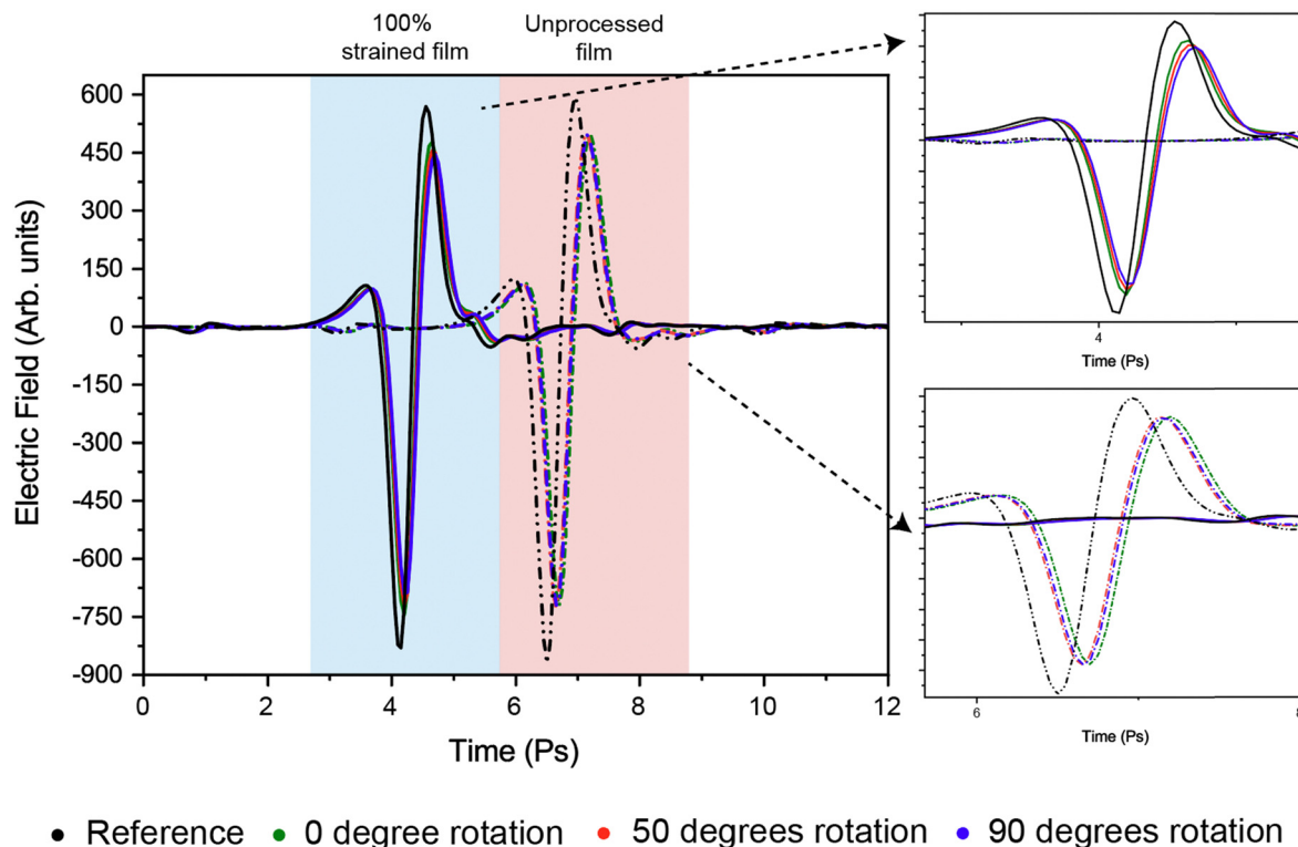
Fig. 3 THz-TDS time trace showing the electric field changes in response to strain and rotation on 100% strained PLLA film and unprocessed PLLA film. The inset provides a detailed magnification.
