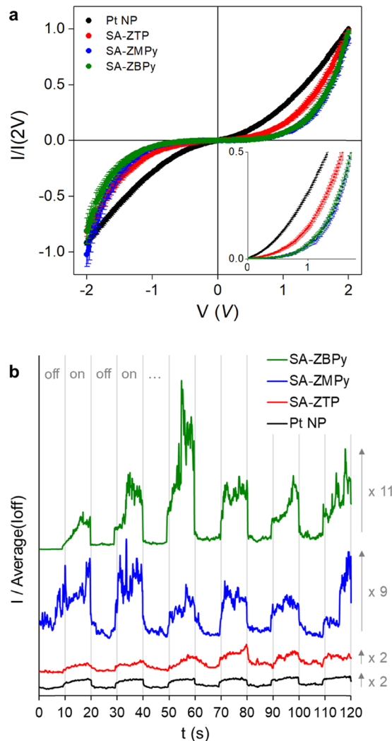
Fig. 5 Charge transport measurements at the nanoscale, performed by conductive AFM on Pt NP , SA-ZTP , SA-ZMPy and SA-ZBPy , at room temperature. (a) I - V curves; the curves are normalized at 2 V; inset: magnification of the 0–1 V region. (b) Evolution of the current intensity under light irradiation at a voltage of 2 V; light is successively switched on and off.
