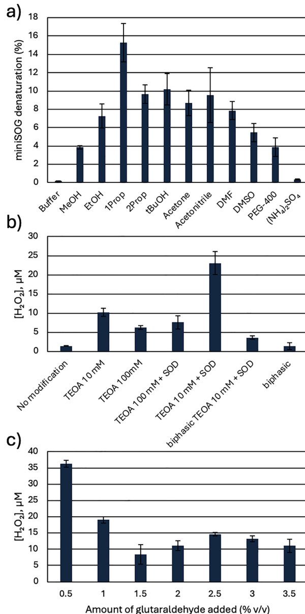
Fig. 2 (a) Precipitant screen. (b) Reaction additive screen. (c) Glutaraldehyde dose optimisation. All data represent mean \pm SD ( n = 3 ). \text{H}_2\text{O}_2 quantification determined by HRP/ABTS assay using a calibration curve (Fig. S6).
