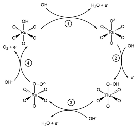
Fig. 11 OER mechanism in lead ruthenate pyrochlores in alkaline media, redrawn with permission from Parrondo et al. 72 Copyright Royal Society of Chemistry 2015.
