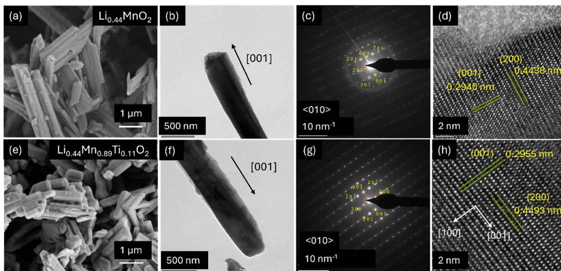
Fig. 3 Morphology analysis. (a) and (e) SEM images of Li 0.44 MnO 2 (LMO1) and Li 0.44 Mn 0.89 Ti 0.11 O 2 (LMO2). (b), (c) and (d) TEM image, SAED pattern and HRTEM image of LMO1. (f), (g) and (h) TEM image, SAED pattern and HRTEM image of LMO2. The \langle 010 \rangle zone axis was taken for the SAED patterns.
