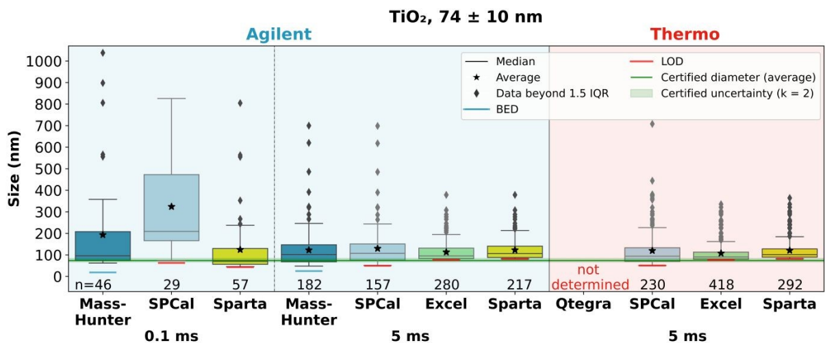
Fig. 5 Size comparison for the ~74 nm TiO 2 NPs via spICP-MS between Agilent (0.1 vs. 5 ms dwell time) and Thermo (5 ms dwell time) using different data processing methods. Two diameters (average, green line) ± uncertainty (green area) were used from the provider's certificate obtained using laser diffraction spectrometry (71 ± 4 nm) and X-ray disc centrifugation (77 ± 7 nm) with a certified expanded uncertainty (k = 2). NP-events were identified above the particle detection threshold (PDT), defined as follows: for the MassHunter software (Agilent), options were set on 'auto' (algorithm not known), for SPCal (set on 'auto', based on the background) the chosen method was Poisson (both instruments and dwell times), and for the Excel (both instruments), the Gaussian method (average (μ) + 7 standard deviations (SDs)) was used. In our case, Sparta used the Poisson method (all data above PDT) for both instruments and dwell times. The Qtegra (Thermo) software was not applied in this round of measurements. 'IQR' = interquartile range. 'LOD' = size limit of detection. 'BED' = background equivalent diameter.
