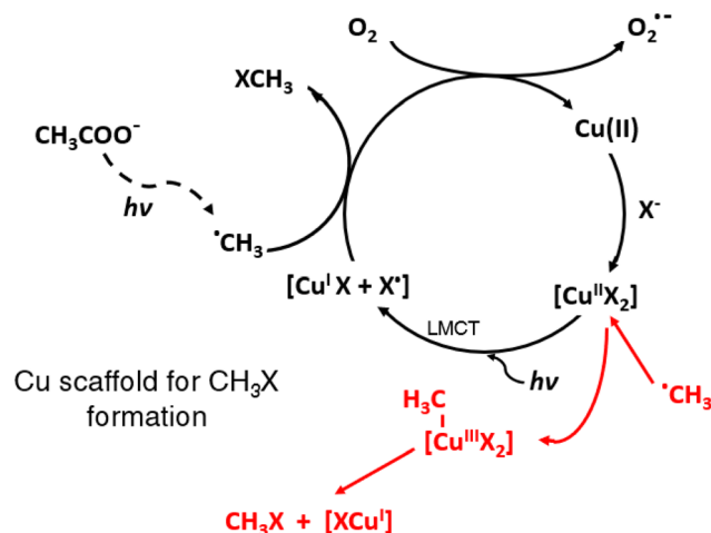
Fig. 1 TM-assisted PVG of halogens using added Cu(II) as an example of aquo-metal halide complex formation followed by (i) \cdot\text{CH}_3 capture of halide atom ( \text{X}\cdot ) formed by a LMCT process or (ii, shown in red) oxidative addition of \cdot\text{CH}_3 to \text{CuX}_2 complex followed by reductive elimination of \text{CH}_3\text{X} and subsequent catalytic re-oxidation of Cu(I) by dissolved oxygen or other oxidants in the system.
