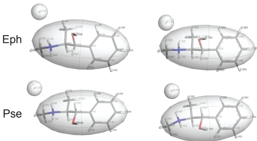
Fig. 4 Motion groups assigned in Module 1 of the QNMRX-CSP protocol for benchmarking calculations, with structural models for Eph (top) and Pse (bottom) based on the known crystal structures (left) and structural models obtained from refining isolated molecules (right).
