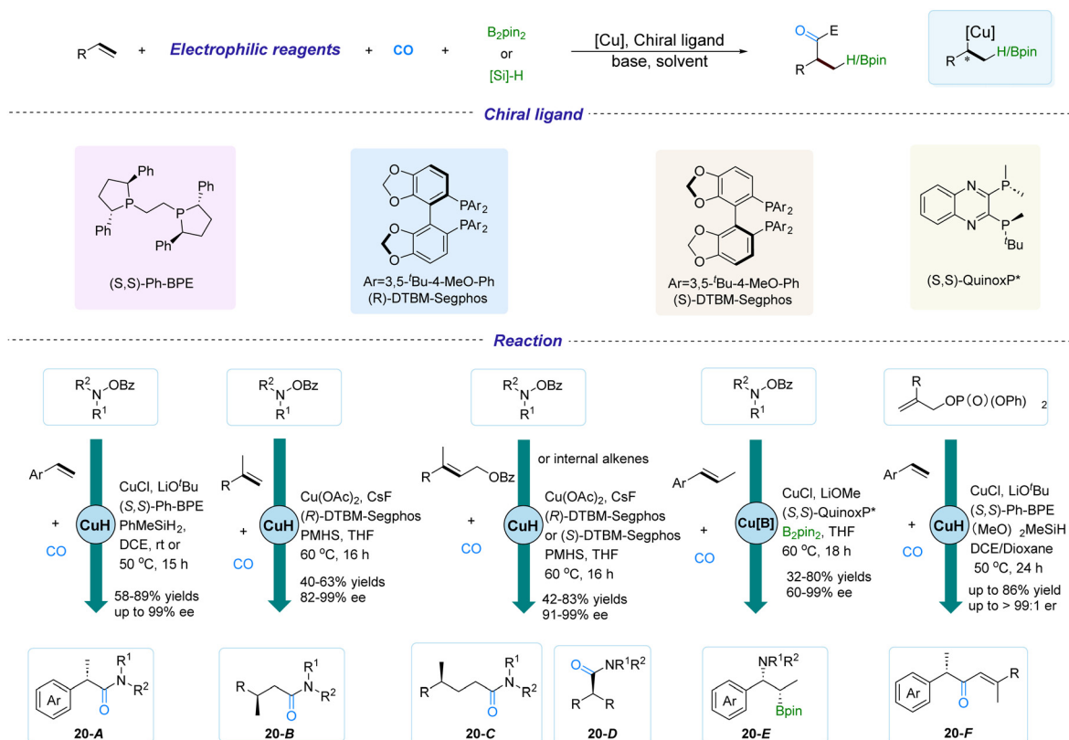
Fig. 20 Organocopper intermediates in the asymmetric carbonylation reaction (Cu–H and Cu–Bpin species addition to alkenes).
