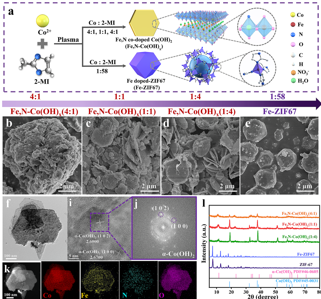
Fig. 1 Preparation process and morphology of electrocatalysts. (a) Schematic of the synthesis of Fe,N co-doped \text{Co(OH)}_2 (i.e., \text{Fe}_x\text{N}_y\text{-Co(OH)}_x ) and Fe-doped ZIF67 (i.e., \text{Fe-ZIF67} ) induced by plasma in water. (b)–(e) SEM images of (b) \text{Fe}_x\text{N}_y\text{-Co(OH)}_x (4 : 1), (c) \text{Fe}_x\text{N}_y\text{-Co(OH)}_x (1 : 1), (d) \text{Fe}_x\text{N}_y\text{-Co(OH)}_x (1 : 4), and (e) \text{Fe-ZIF67} . (f)–(k) Morphology and elemental distribution of \text{Fe}_x\text{N}_y\text{-Co(OH)}_x (1 : 1): (f) TEM images, (i) HAADF-STEM images, (j) corresponding FFT pattern, and (k) EDS mapping images. (l) XRD patterns of \text{Fe}_x\text{N}_y\text{-Co(OH)}_x (4 : 1) (orange line), \text{Fe}_x\text{N}_y\text{-Co(OH)}_x (1 : 1) (red line), \text{Fe}_x\text{N}_y\text{-Co(OH)}_x (1 : 4) (green line), and \text{Fe-ZIF67} (purple line).
