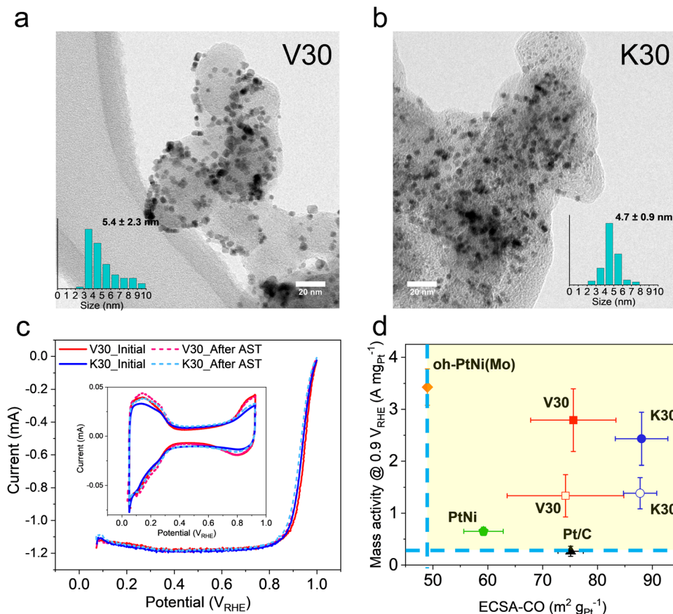
Fig. 2 TEM images of (a) V30 and (b) K30. In the inset is the histogram for nanoparticle size. (c) RDE LSV of V30 and K30, scanning rate 20 mV\ s^{-1} . The solid lines represent the LSV before the AST, 10k cycles between 0.6 to 0.925 V_{RHE} , scanning rate 100 mV\ s^{-1} ; the dashed lines for the LSV after AST. In the inset, the cyclic voltammetry for V30 and K30 is shown, before and after the AST. RDE measured in 0.1 M HClO_4 . (d) Mass activity measured at 0.9 V_{RHE} of V30 and K30 in RDE as a function of corresponding ECSA-CO before and after AST. Solid symbols are initial electrochemical performance; hollow symbols denote results after AST. V30 sample is marked as a red square; the K30 sample is a blue circle; oh-PtNi(Mo) is a yellow diamond; Pt/C is a black triangle; PtNi reference is a green pentagon. Data for oh-PtNi(Mo) adapted from ref. 9. Solid symbols represent the catalytic performance at the beginning of life (BoL) and after AST, the hollow symbols show the performance at the end of life (EoL).
