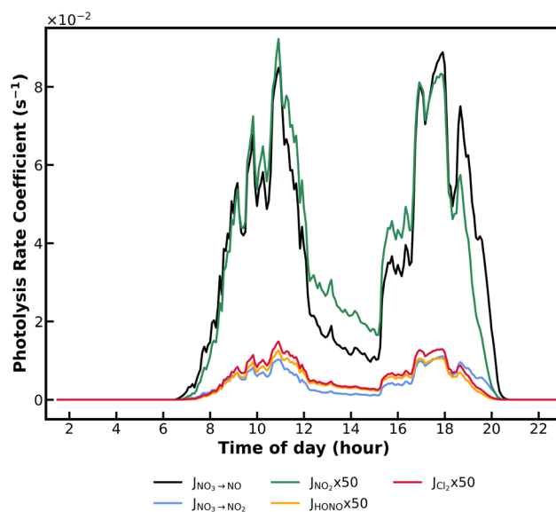
Fig. 1 Selected average photolysis rate coefficients ( J ) from measurements located both in the kitchen and living room, representing the outdoor attenuated light experienced inside the house: J NO 3 →NO (black line), J NO 3 →NO 2 (blue line), J NO 2 × 50 (green line), J HONO × 50 (yellow line), and J Cl 2 × 50 (red line).
