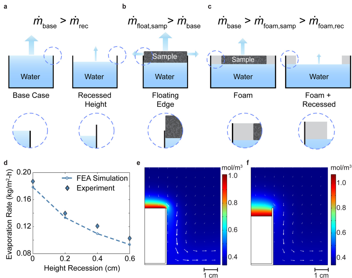
Fig. 2 Effects of experimental setup on apparent measured evaporation rates. (a) \dot{m}_{base} is the base case rate when pure water is leveled with container lip, \dot{m}_{rec} is for water recessed below the lip. (b) \dot{m}_{float,samp} represents the case when the porous floating sample top surface rises above the container lip. Evaporation from the side leads to a higher apparent rate than \dot{m}_{base} . (c) \dot{m}_{foam,samp} is the rate when foam insulation wraps around the sample during evaporation experiments, which is lower than \dot{m}_{base} as the edge effect is reduced in the former. \dot{m}_{foam,rec} represents the rate with foam in the absence of sample, which is even lower due to the recessed water level. (d) Effects of recessed evaporating surface on evaporation rates from FEA simulations (blue dashed line) and experiments (blue diamonds). Simulations are conducted for 30% RH at 23 °C. Experiments are conducted in 31.1 \pm 1.1\% RH at 24.58 \pm 0.15 °C. FEA snapshots of the vapor concentration distribution and natural convection velocity magnitudes evaporating into 30% RH and 23 °C ambient with the water surface (e) leveled with the container lip and (f) 6 mm below the container lip. Arrow lengths are normalized linearly to the largest velocity seen in both simulations.
