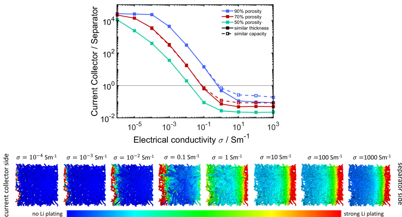
Fig. 5 Top: influence of electrical conductivity on the ratio of the effective, mean amount of Li plating on the current collector and separator sides in microstructures with different porosities (train 11 635, train 5481, and train 44 842; cf. Table S3†) but similar thickness/capacity after 10 s at 0.1 \text{ mA cm}^{-2} . An extended figure which additionally includes a dual-layer structure with a surface area and porosity gradient can be found in the ESI (Fig. S16†). Bottom: the amount of plated Li on a highly porous (90%) fiber system (train 11 635, cf. Table S3†) with electrical conductivities of \sigma = 10^{-4} – 10^3 \text{ S m}^{-1} after 10 s at 0.1 \text{ mA cm}^{-2} . The shown view is from the side in the through direction. The current collector is located on the left side, while the separator is beginning on the right. An extended figure including all three structures with different porosities can be found in the ESI (Fig. S15†).
