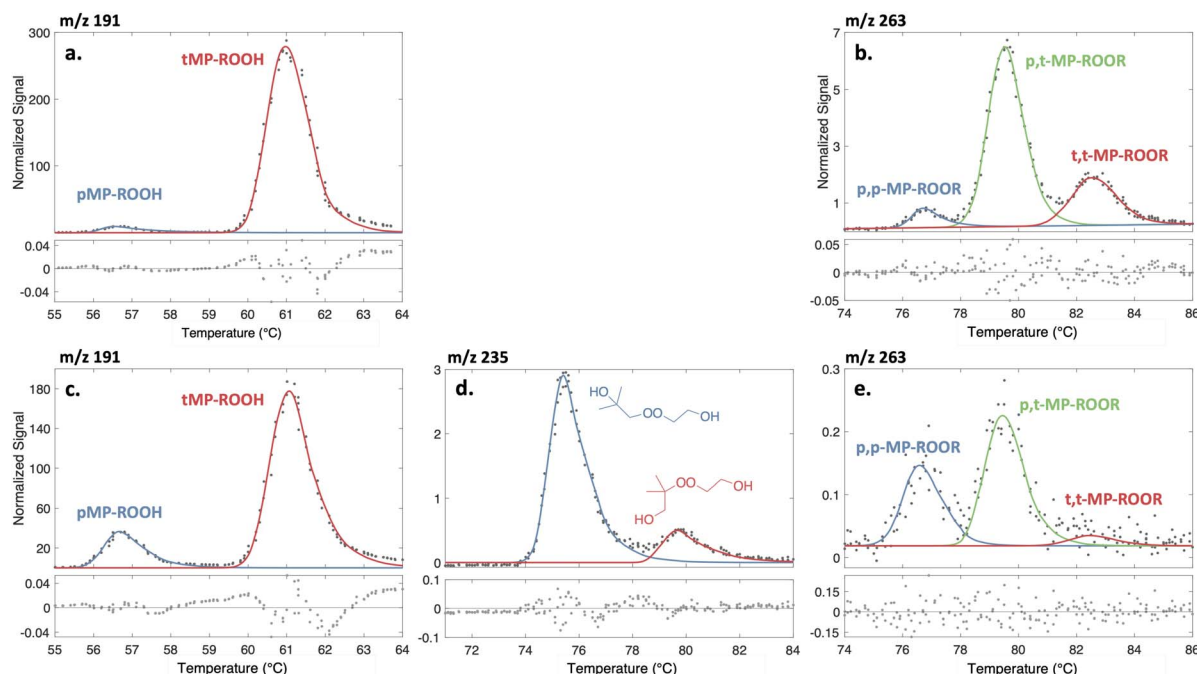
Fig. 1 Representative chromatograms of ROOH (a and c) and ROOR (b, d, and e) products formed in the oxidation of 2-methylpropene in experiments with high RO_2/HO_2 ratios (top row) and high HO_2/RO_2 ratios (bottom row). Experiments represented in the bottom row also included ethene. The experimentally measured signal is given as dark gray dots, while the colored lines are the bootstrap best fits of the chromatographic data. The corresponding structures are the assignments of these peaks. Below each chromatogram are plots of the residuals of the best fits given as fractions of the maximum peak value.
