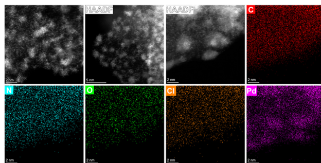
Fig. 5 HAADF-STEM images and the corresponding elemental mapping of POP-Tpy-1-Pd.
