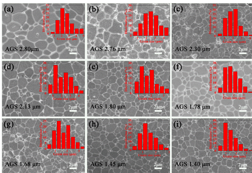
Fig. 2 The typical SEM morphologies of the (0.36 - x )PNN- x PMN-0.28PZ-0.36PT:0.02Sm ceramics: (a) x = 0 , (b) x = 0.03 , (c) x = 0.06 , (d) x = 0.09 , (e) x = 0.12 , (f) x = 0.15 , (g) x = 0.18 , (h) x = 0.21 , and (i) x = 0.24 .
