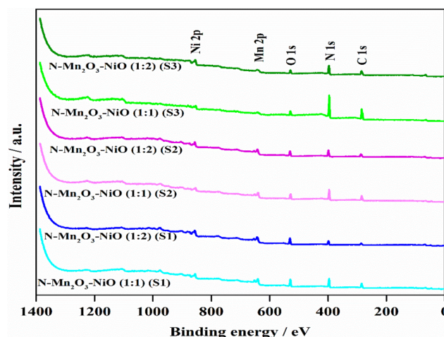
Fig. 2 XPS general spectrum of synthesised N-Mn 2 O 3 -NiO structures.
